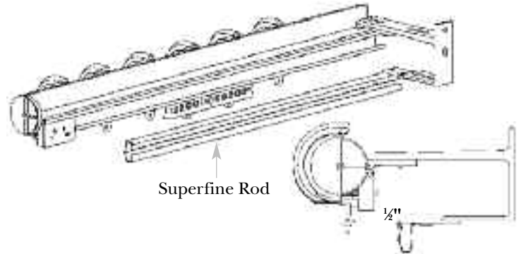
Double Treatment with 71132 Bracket
